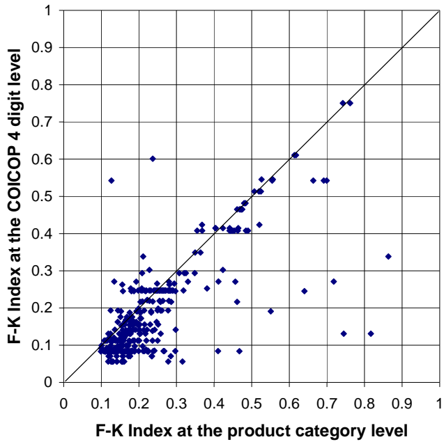
Scatter plots of the F-K index of price changes (full sample)
